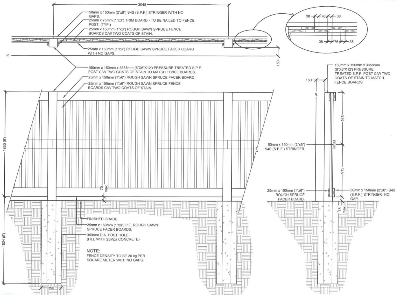
1 1800mm HT. OVERLAP WOOD SCREEN FENCE SCALE: 1:20
