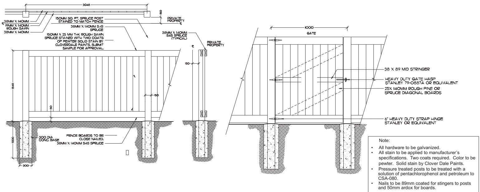
1 1.8m STANDARD WOOD SCREEN FENCE AND GATE L07 SCALE: N.T.S.
