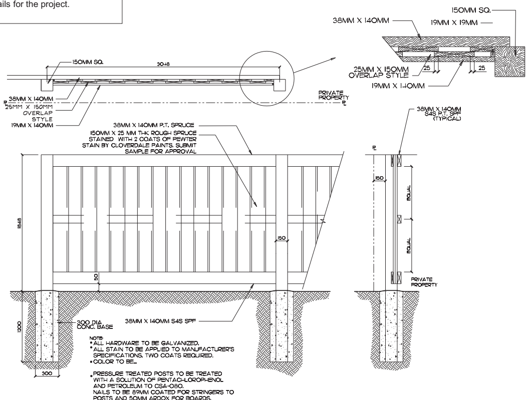
4 OVERLAP BOARD WOOD SCREEN FENCE L07 SCALE: N.T.S.
